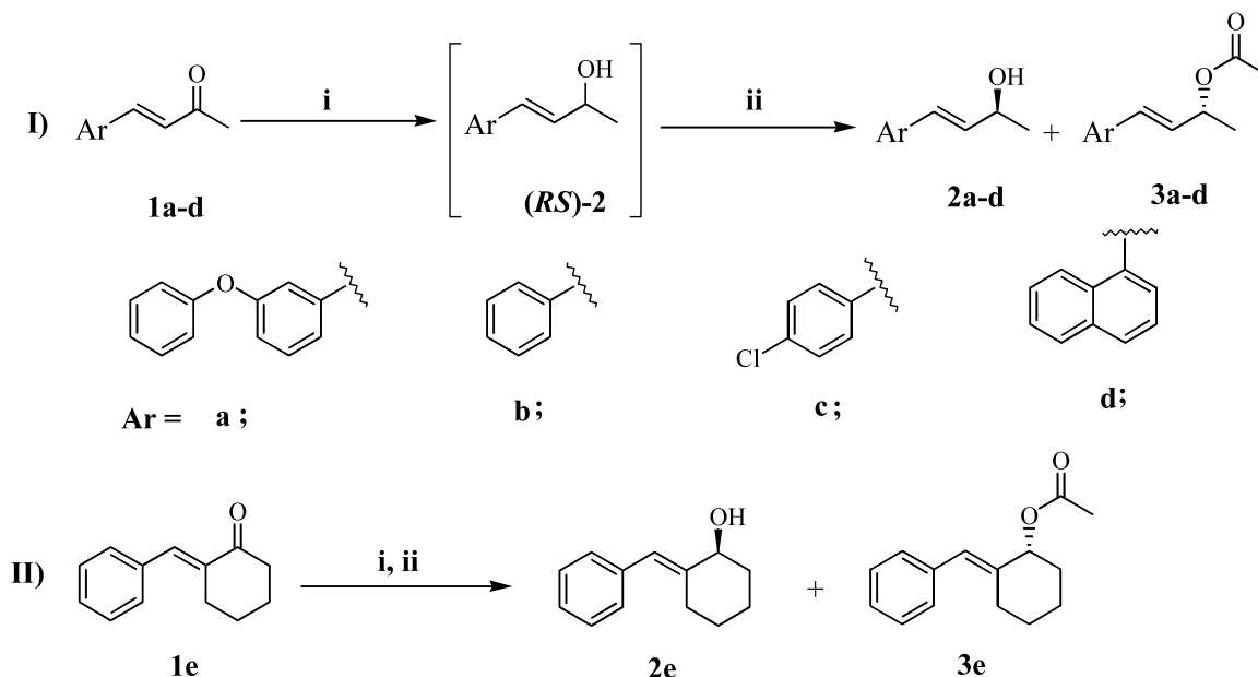
Scheme 1. Reagents and conditions: (i) \text{NaBH}_4 , activated alumina, diisopropyl ether; (ii) Lipase PS-C 'Amano' II, isopropenyl acetate.
